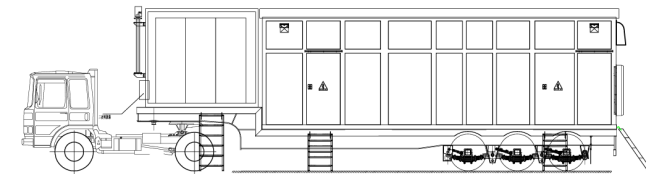
Distribution Trailer
