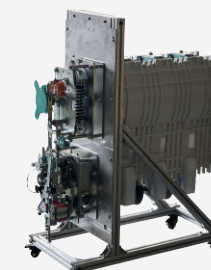
24kV Vacuum Circuit Breaker for Dry-air insulated RMU
