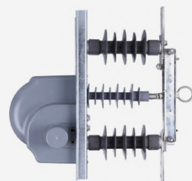
Motorized Disconnecter
